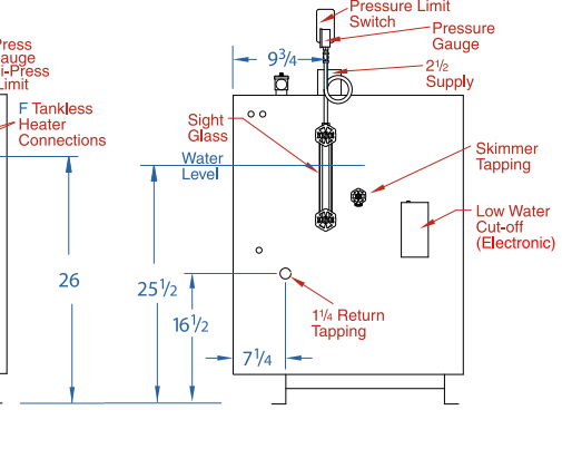
RIGHT SIDE VIEW GXH PZ Steam Models
