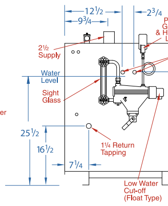
RIGHT SIDE VIEW GXH PZT, PPZT Steam Models
